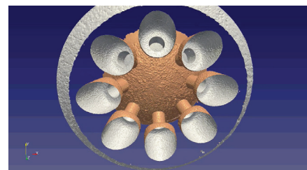
Cut-through images of a fuel injector, as shown with X-ray tomography. Interior nozzle hole size of roughly 170 microns. Tomography gives precise measurement (with no damage) of the as-built injector. Knowledge of nozzle defects is crucial in understanding fuel-injection behavior.
